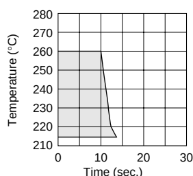
Allowable Flow Soldering Temperature and Time
