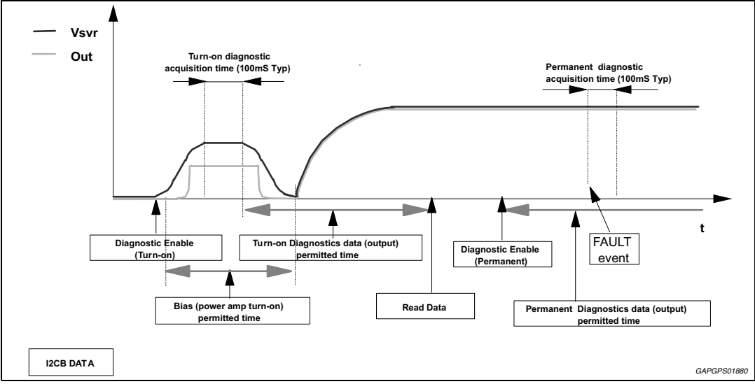
Figure 21. SVR and output pin behavior (case 2: with turn-on diagnostic)
