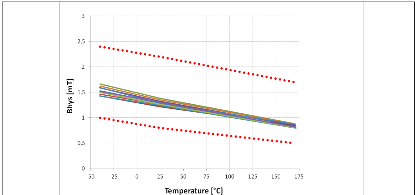
Figure 5-3 Hysteresis ( B_{Hys} ) of the TLE4964-4M over Temperature
