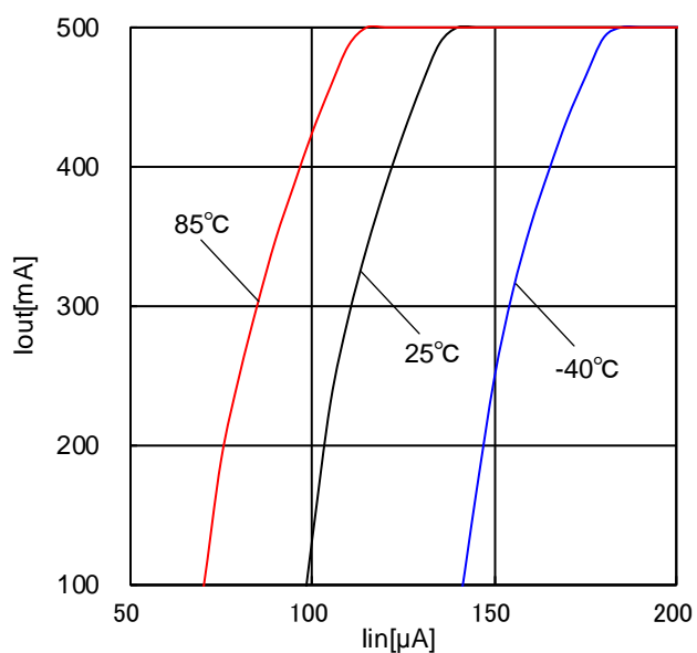
Figure 3 . Output Current vs Input Current
