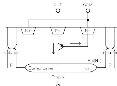
Figure 19. Construction of output clamp diode
