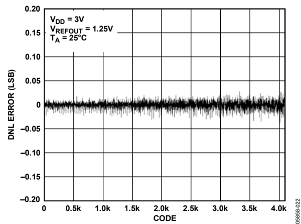
Figure 21. DNL AD5623R-3
