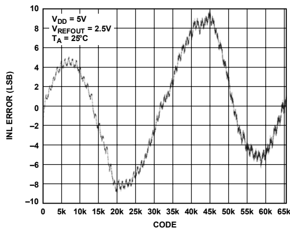
Figure 10. INL AD5663R-5
