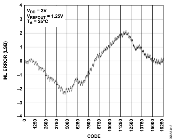
Figure 17. INL AD5643R-3
