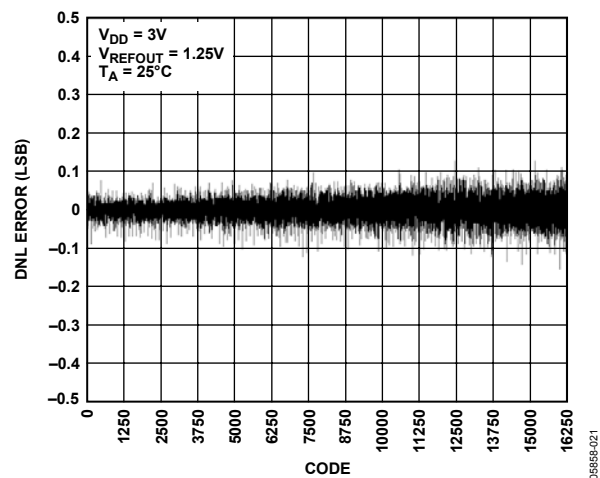
Figure 20. DNL AD5643R-3
