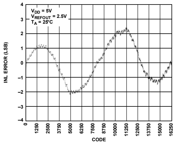
Figure 11. INL AD5643R-5
