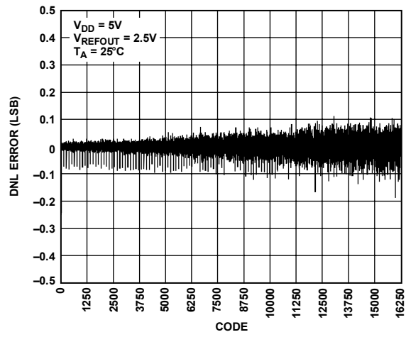
Figure 14. DNL AD5643R-5
