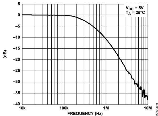
Figure 47. Multiplier Bandwidth
