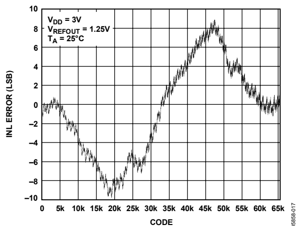
Figure 16. INL AD5663R-3
