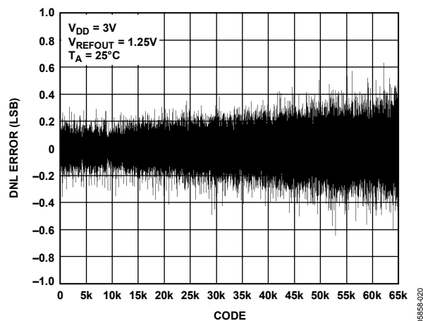
Figure 19. DNL AD5663R-3
