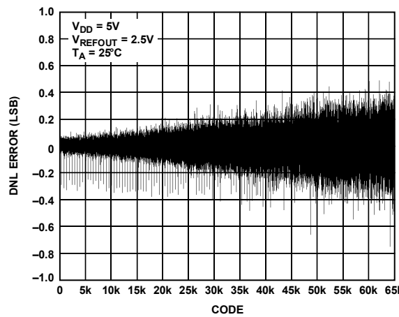
Figure 13. DNL AD5663R-5
