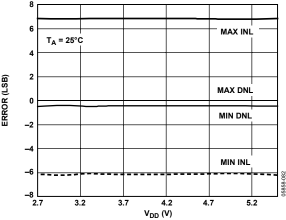
Figure 24. INL and DNL Error vs. Supply
