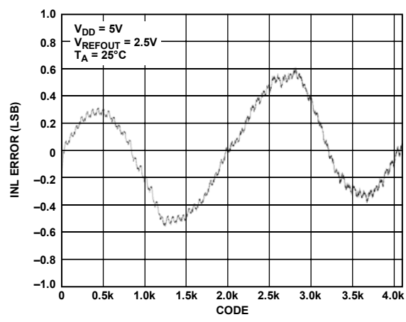
Figure 12. INL AD5623R-5
