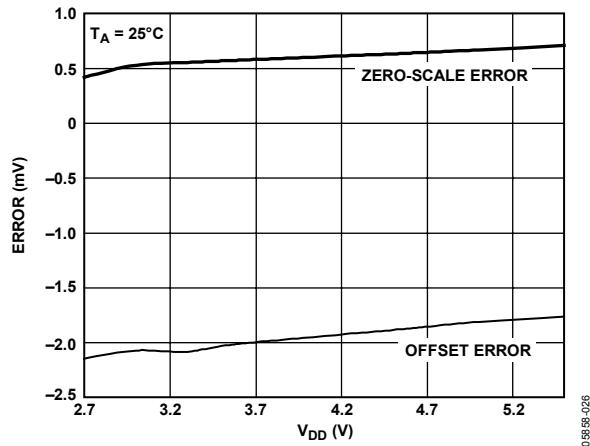
Figure 28. Zero-Scale and Offset Error vs. Supply
