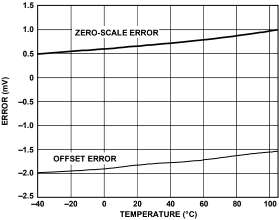
Figure 26. Zero-Scale and Offset Error vs. Temperature
