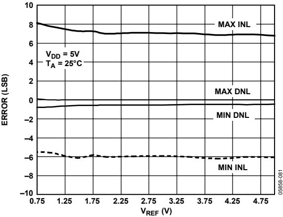
Figure 23. INL and DNL Error vs. V_{REF}
