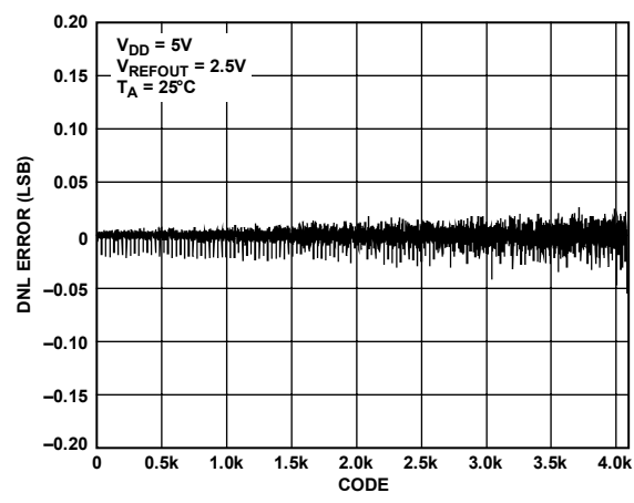
Figure 15. DNL AD5623R-5
