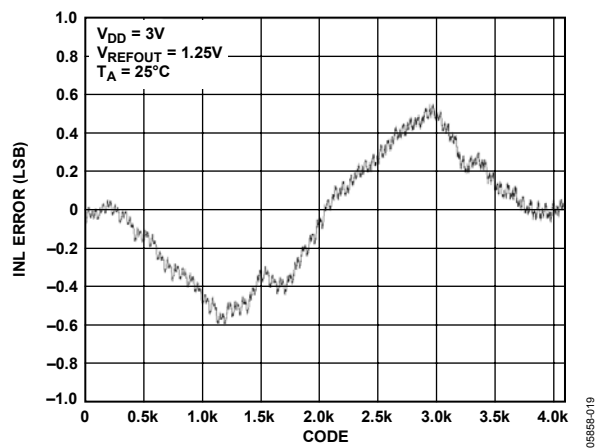
Figure 18. INL AD5623R-3
