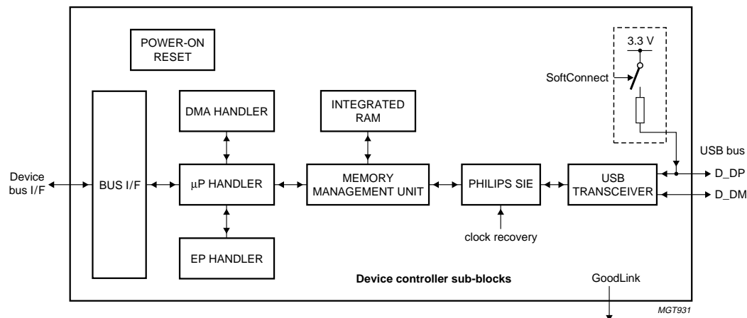
Fig 6. Device controller sub block diagram.
