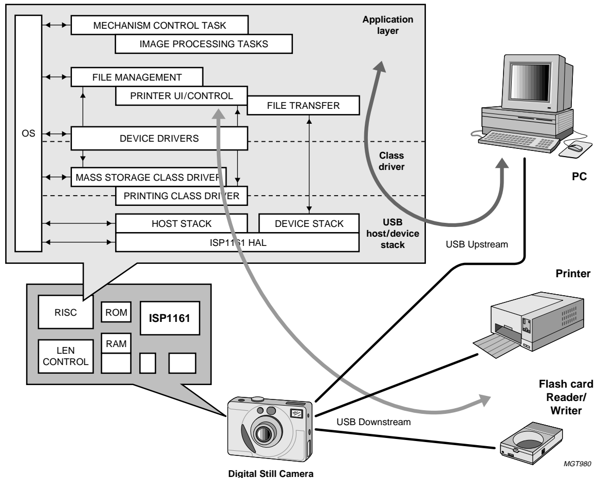
Fig 56. ISP1161 software model for DSC application.
