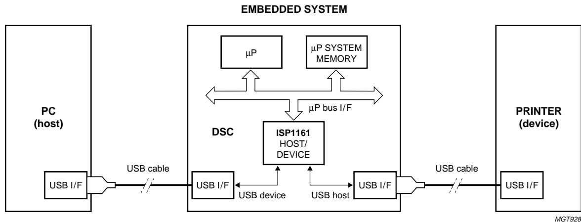
Fig 3. ISP1161 operating as both USB host and device simultaneously.
