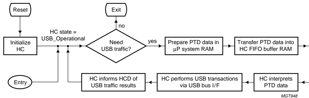
Fig 24. ISP1161 HC operating flow.
