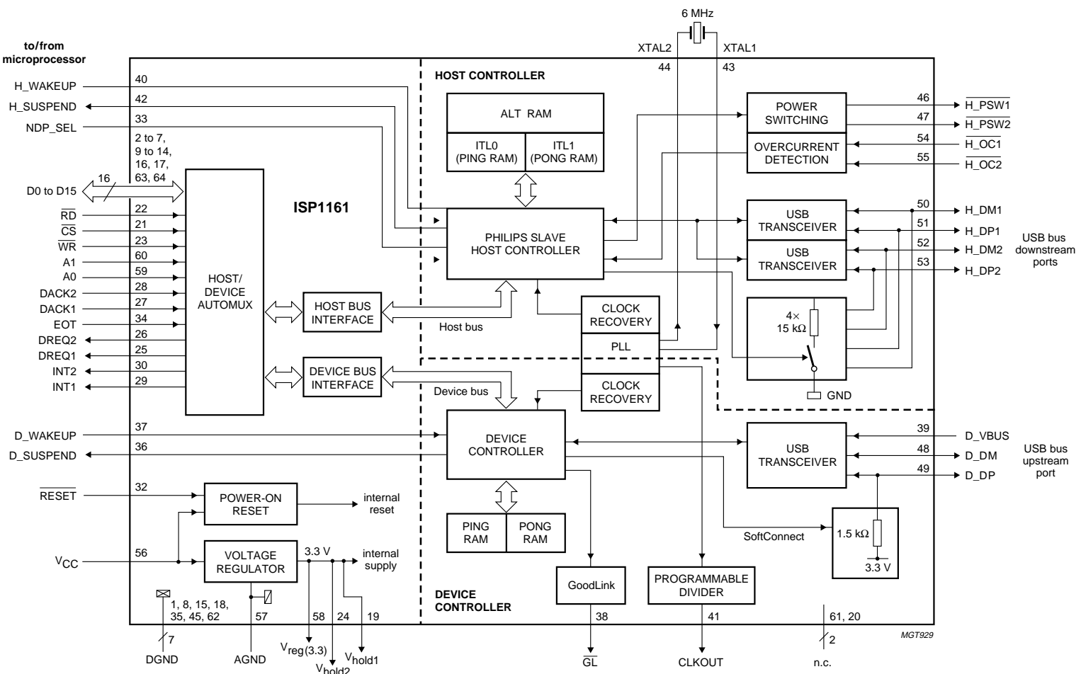
Fig 4. Block diagram.
