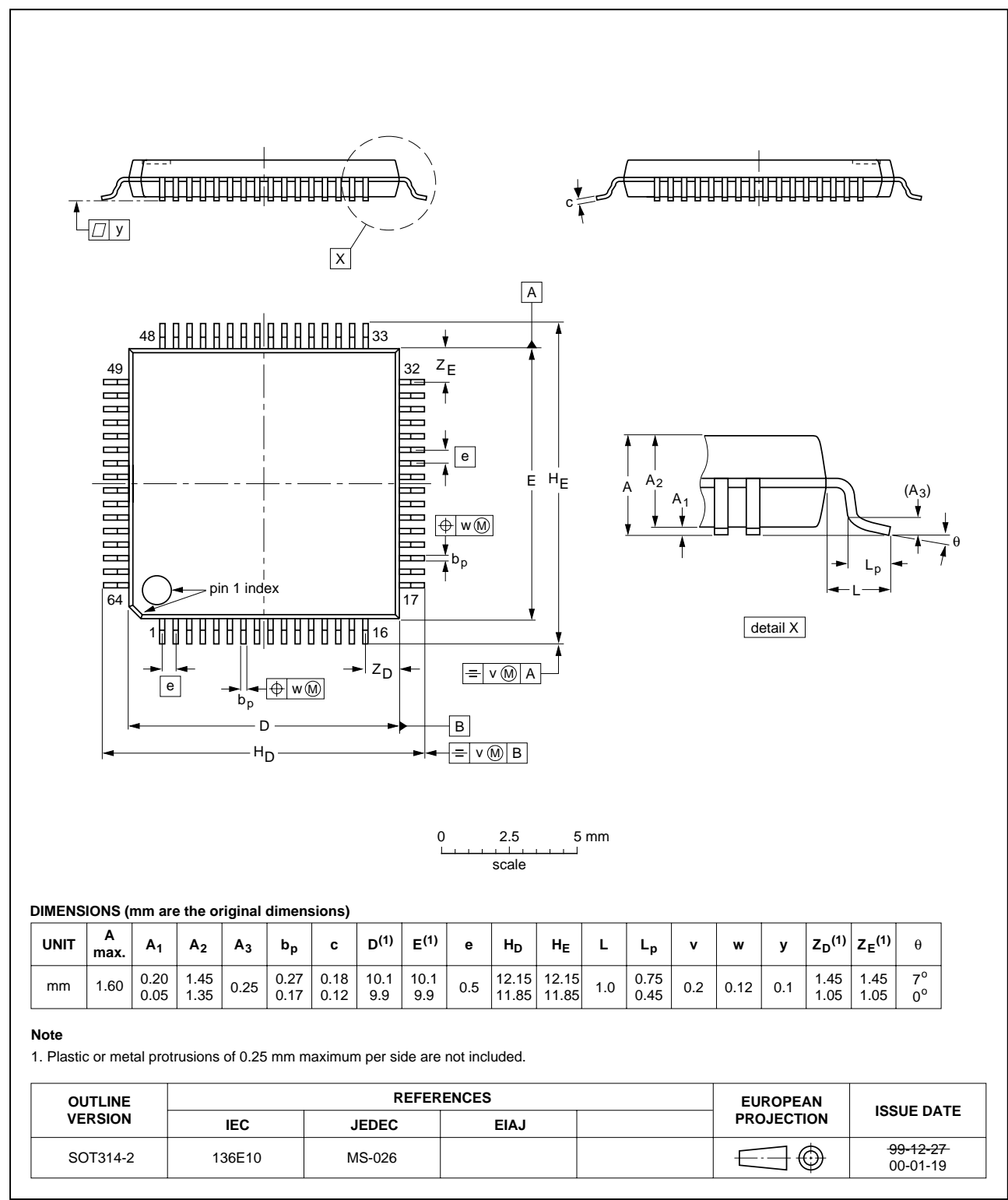
Fig 58. LQFP64 (SOT314-2) package outline.
