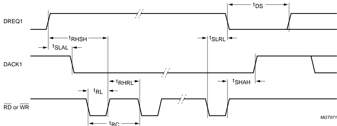
Fig 47. HC multi-cycle burst mode DMA timing.
