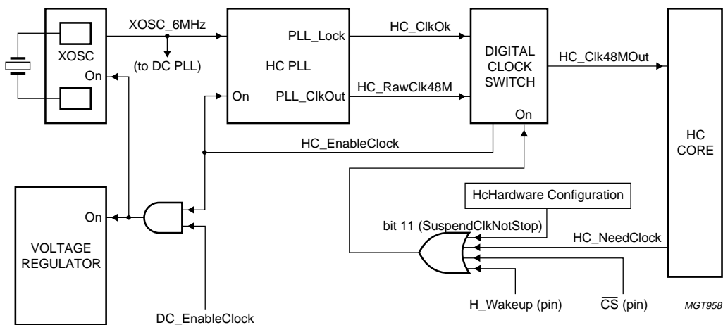
Fig 37. ISP1161 suspend and resume clock scheme.
