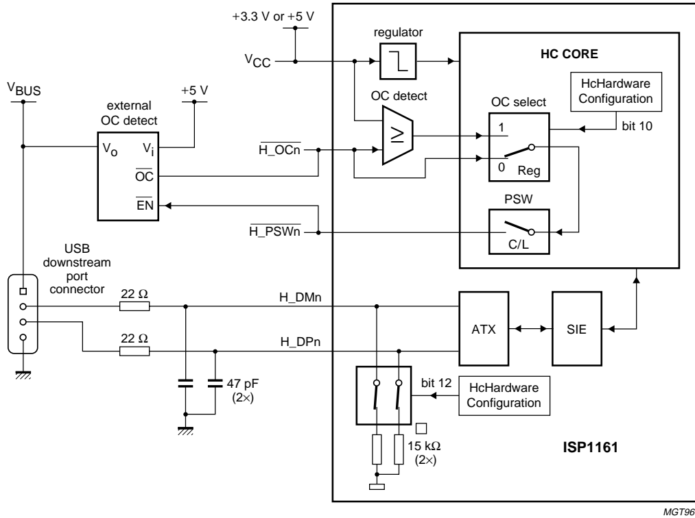
Fig 36. Using external OC detection circuit.
