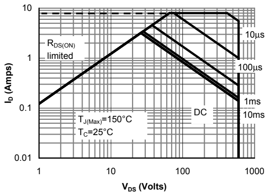
Figure 9: Maximum Forward Biased Safe Operating Area for AOT3N60 (Note F)
