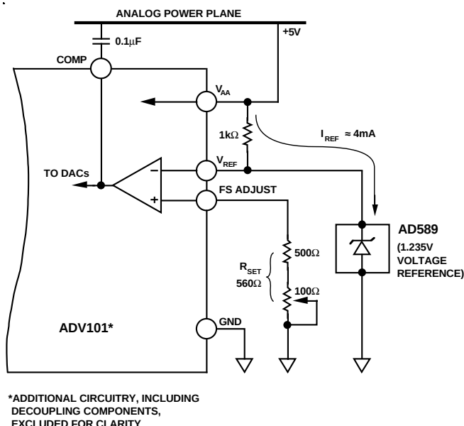
Figure 4. Reference Circuit
