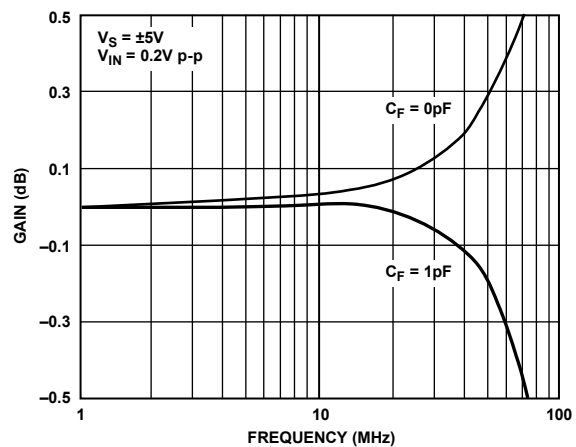
Figure 7. 0.1 dB Flatness vs. Frequency
