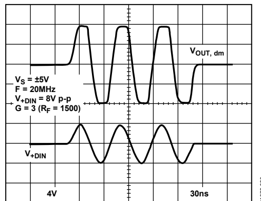
Figure 26. Output Overdrive
