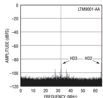
64k Point FFT, f_{IN} = 162.4\text{MHz} , -1dBFS, PGA = 1
