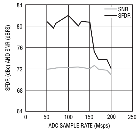
SFDR and SNR vs Sample Rate, f_{IN} = 162.4\text{MHz} , -1\text{dBFS} , \text{PGA} = 0 , \text{RAND} "Off", \text{Dither} = \text{"Off"}
