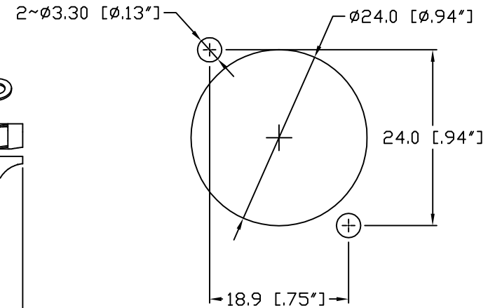
PANEL CUT OUT
