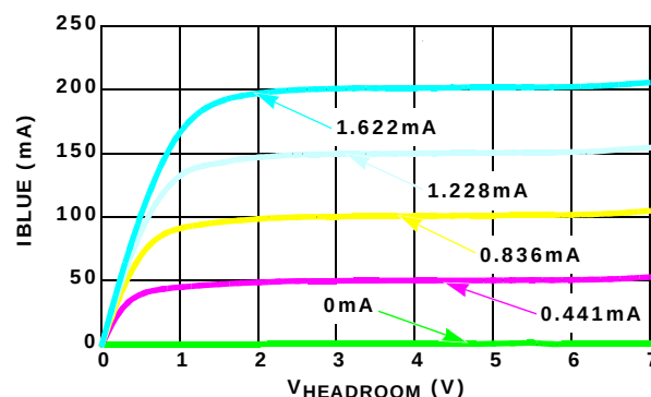
FIGURE 4. I_{\text{BLUE}} READ vs V_{\text{HEADROOM}} vs I_{\text{APC}} , (REG 1-21 = 88h) ( V_{\text{SO}} = 5.0\text{V} ), ( R_{\text{SET}} = 620\Omega )
