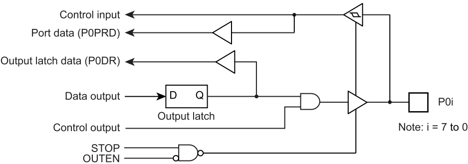
Figure 5-2 Port P0
