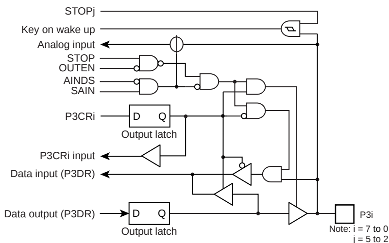
Figure 5-5 Port P3
