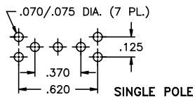
FRONT VIEW SINGLE POLE
