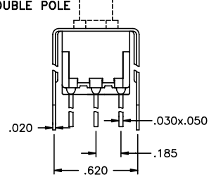
PRINTED CIRCUIT MOUNTING
