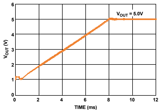
FIGURE 31. TURN-ON TIME
