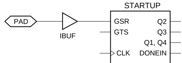
Figure 19: Schematic Symbols for Global Set/Reset
