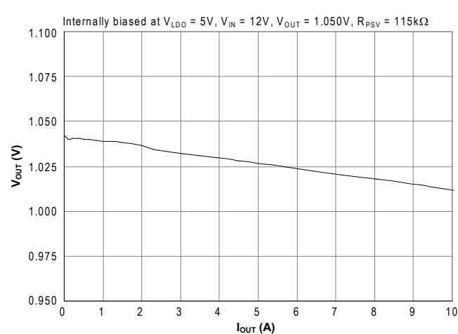
V_{OUT} vs. Load — Ultrasonic Power-save Mode
