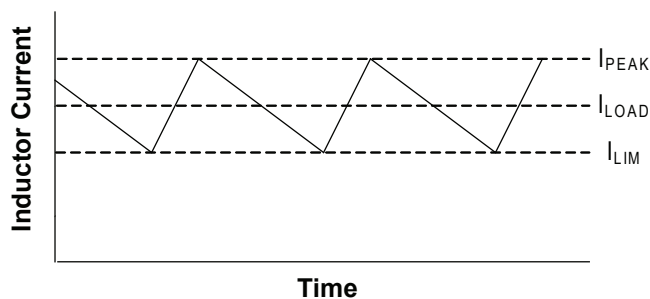
Figure 8 — Valley Current Limit
