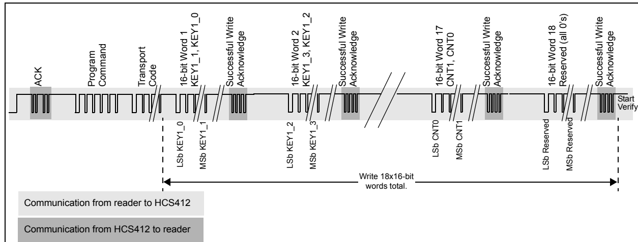
FIGURE 4-10: PROGRAMMING - VERIFICATION
