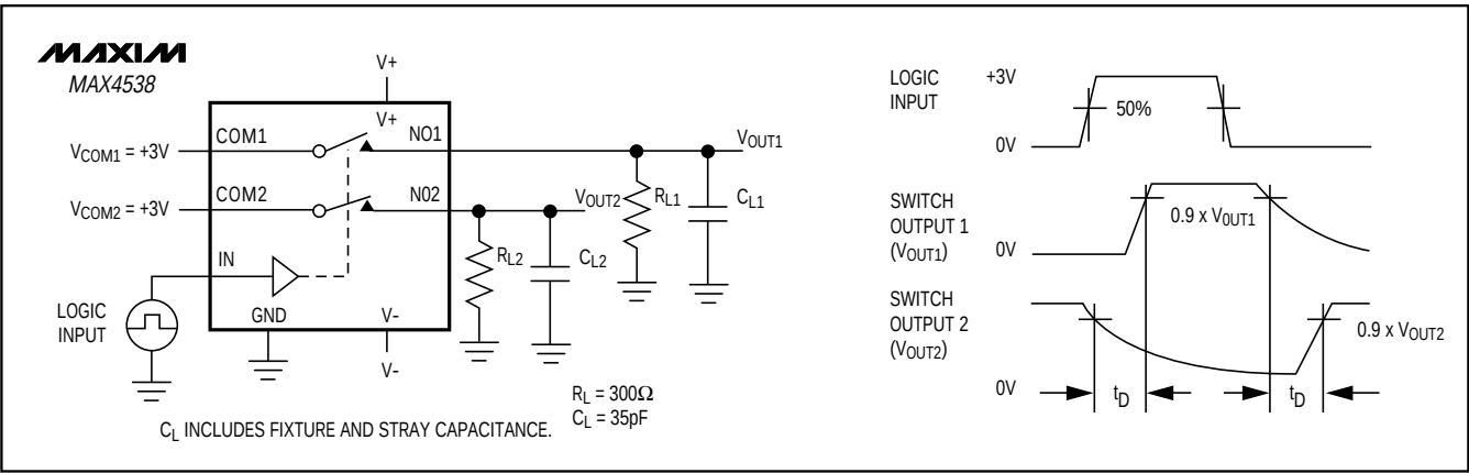
Figure 2. Break-Before-Make Interval (MAX4538 only)
