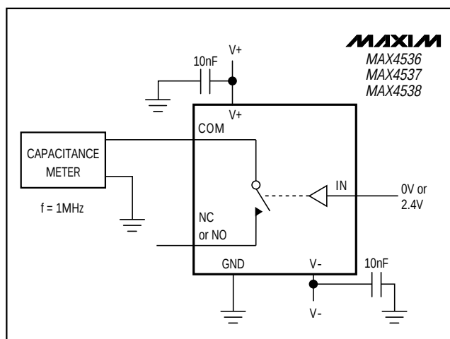
Figure 7. Channel-On Capacitance
