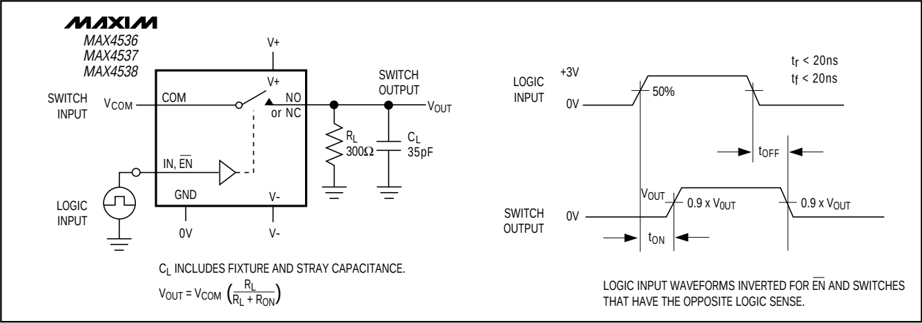
Figure 1. Switching Time
