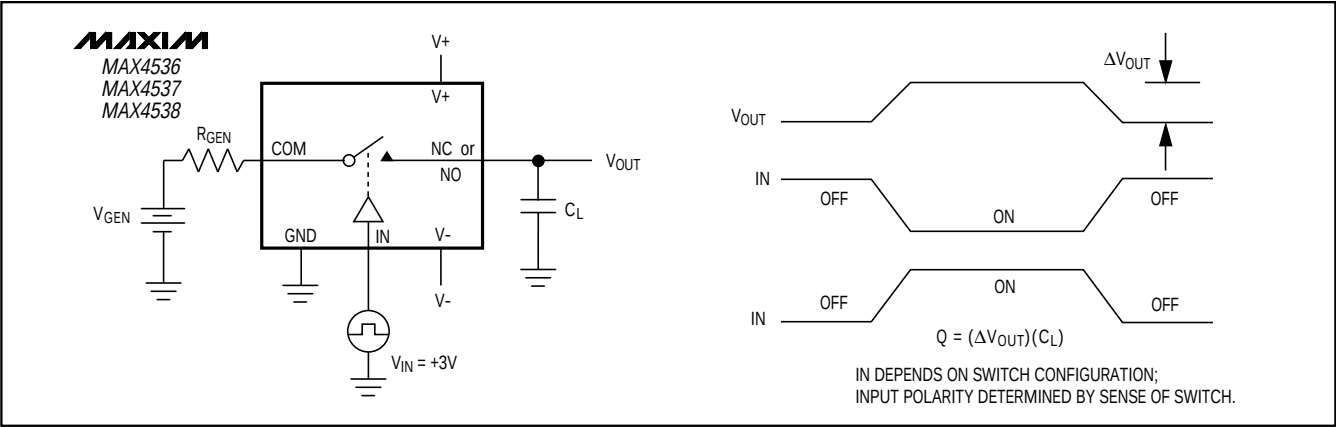
Figure 3. Charge Injection
