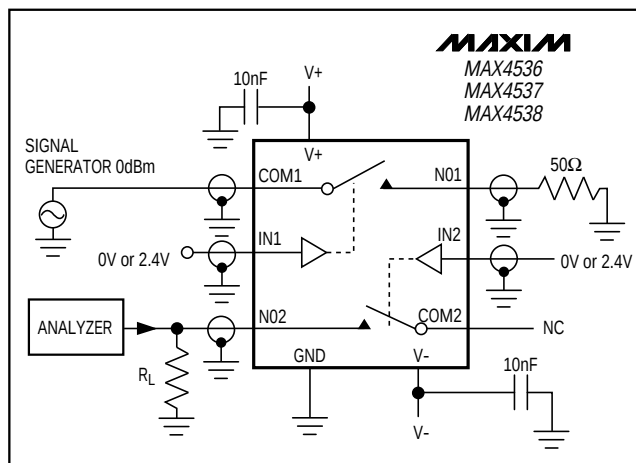
Figure 5. Crosstalk
