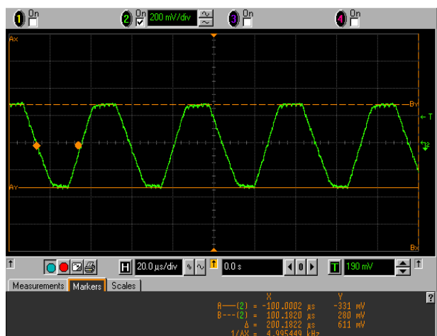
FIGURE 12. 22kHz TONE ON 13.3V_OUT WITH 500mA LOAD
