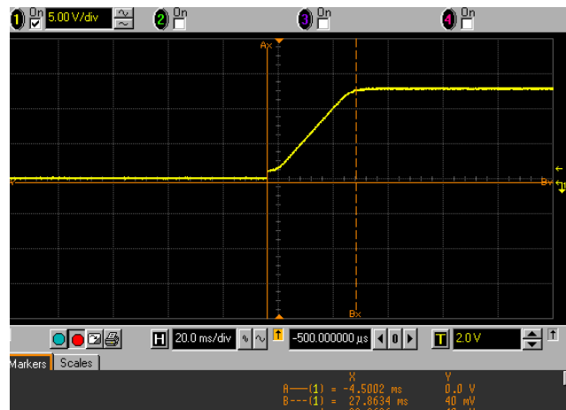
FIGURE 5. V_LNB RISE TIME WITH T_CAP = 0.44 μF is 32ms
