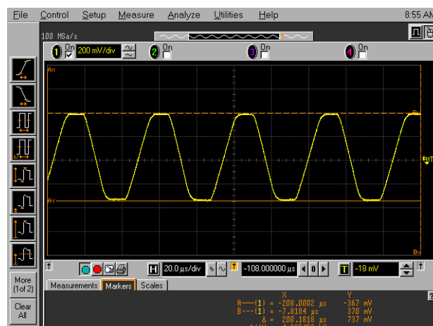
FIGURE 11. 22kHz TONE ON 13.3V_OUT WITH 50mA LOAD
