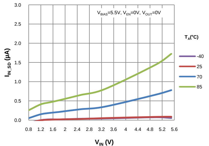
V_{\text{IN}} vs. OFF-STATE V_{\text{IN}} CURRENT (SINGLE CHANNEL)
