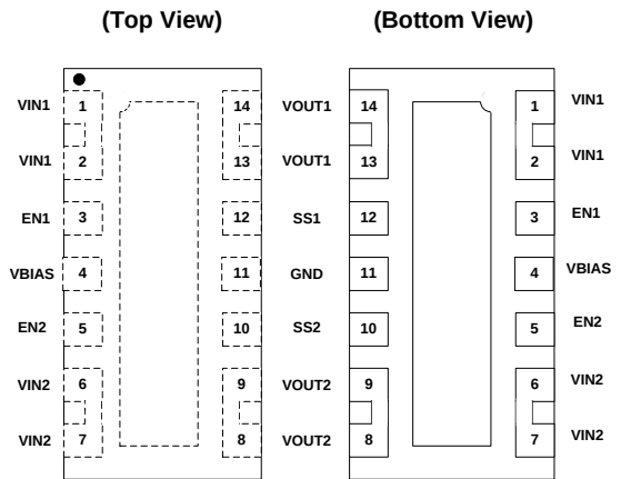
V-DFN3020-14
