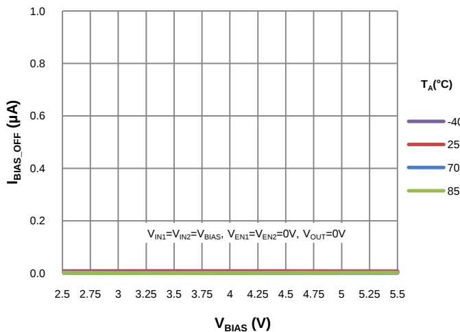
V_{\text{BIAS}} vs. SHUTDOWN CURRENT (BOTH CHANNELS)
