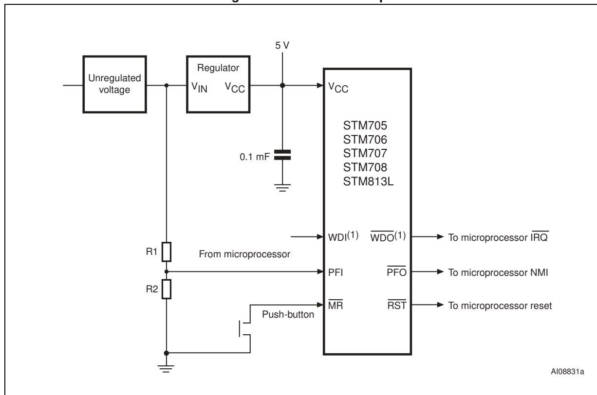
Figure 9. Hardware hookup
