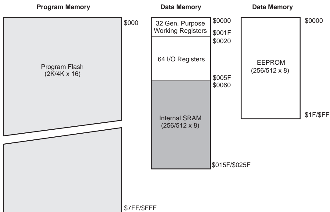
Figure 4. Memory Maps
