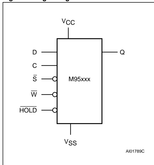
Figure 1. Logic Diagram
