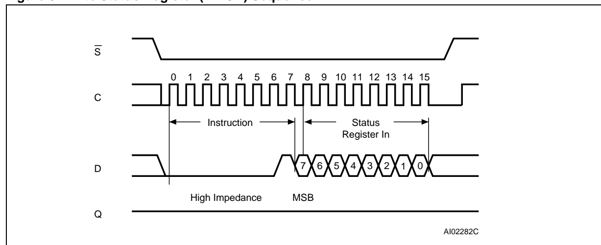
Figure 8. Write Status Register (WRSR) Sequence
