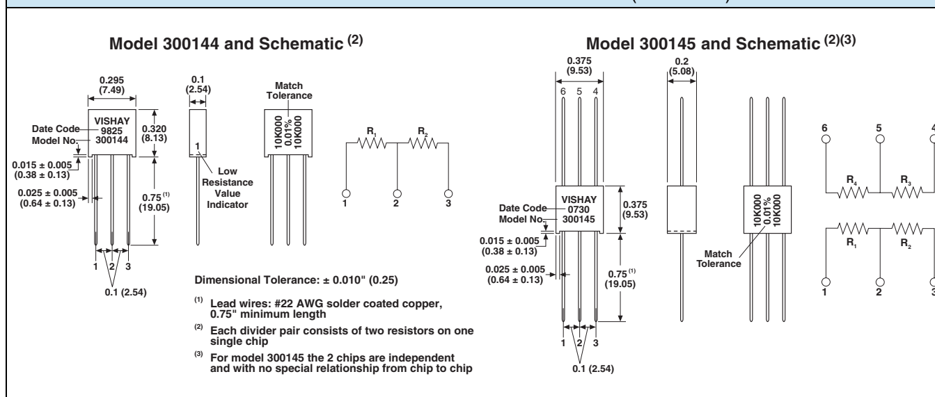
FIGURE 2 - STANDARD PRINTING AND DIMENSIONS in inches (millimeters)
