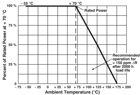
FIGURE 3 - POWER DERATING CURVE 300144, 300145
