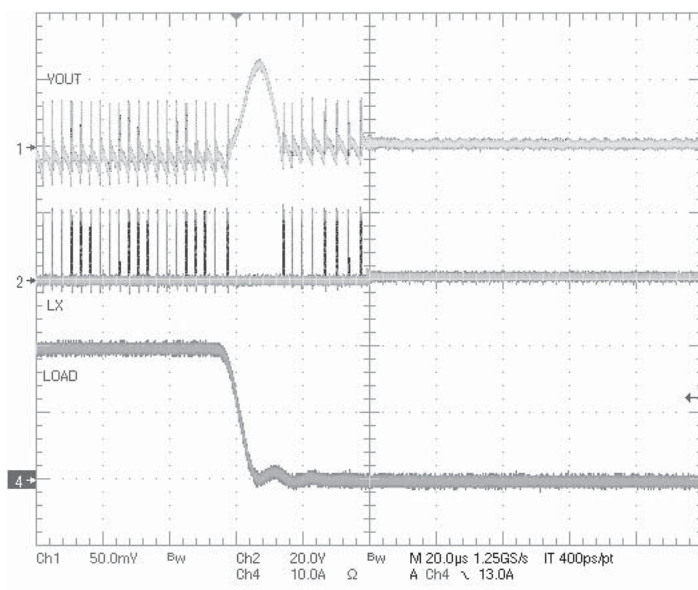
Load Transient Response 20A to 0A
