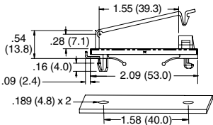
Mounting Holes
