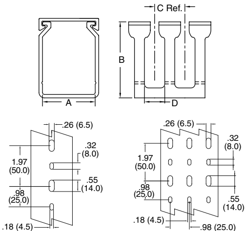
Mounting Style 1
