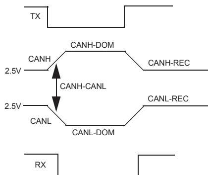
Figure 35. CAN Driver Operation in Normal Mode
