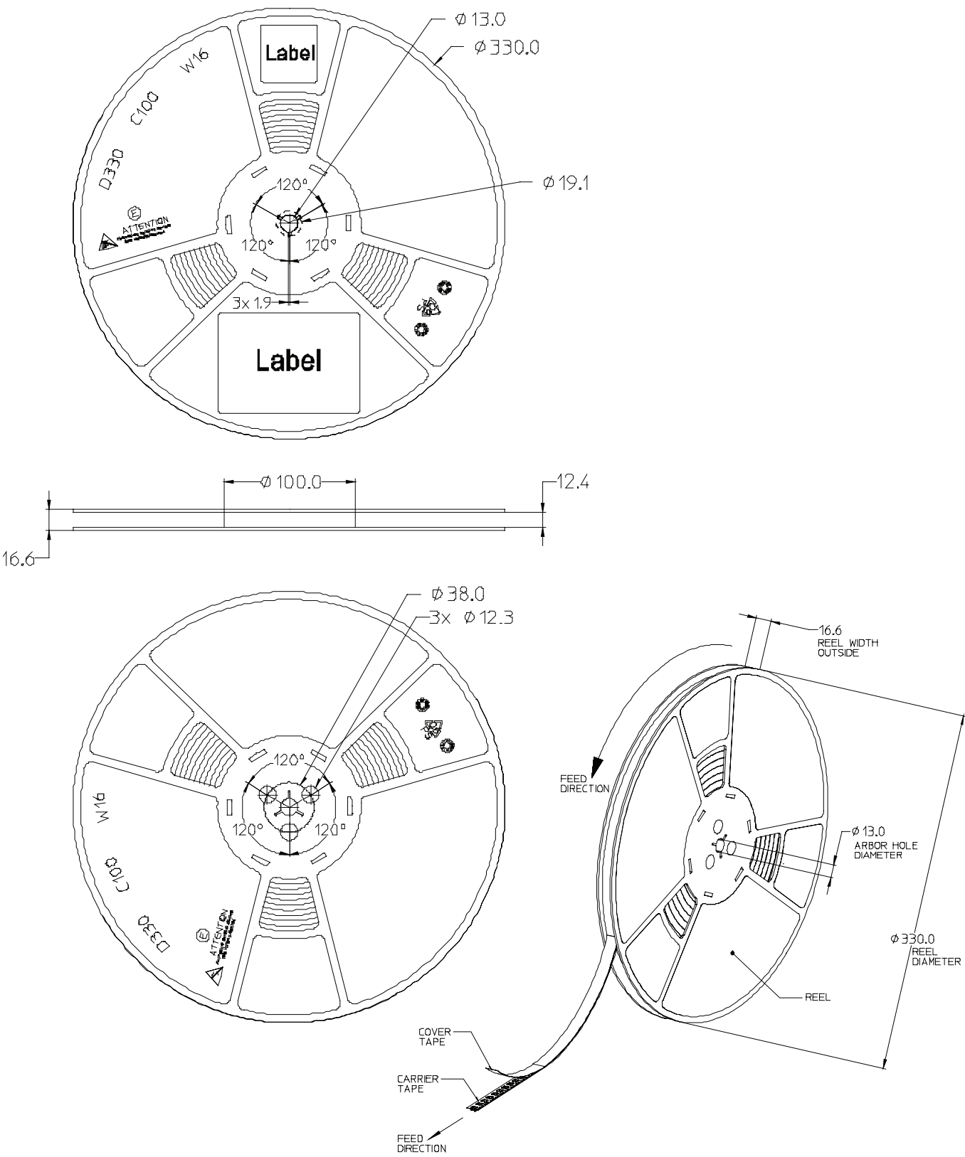
Figure 37. Emitter reel packaging.
