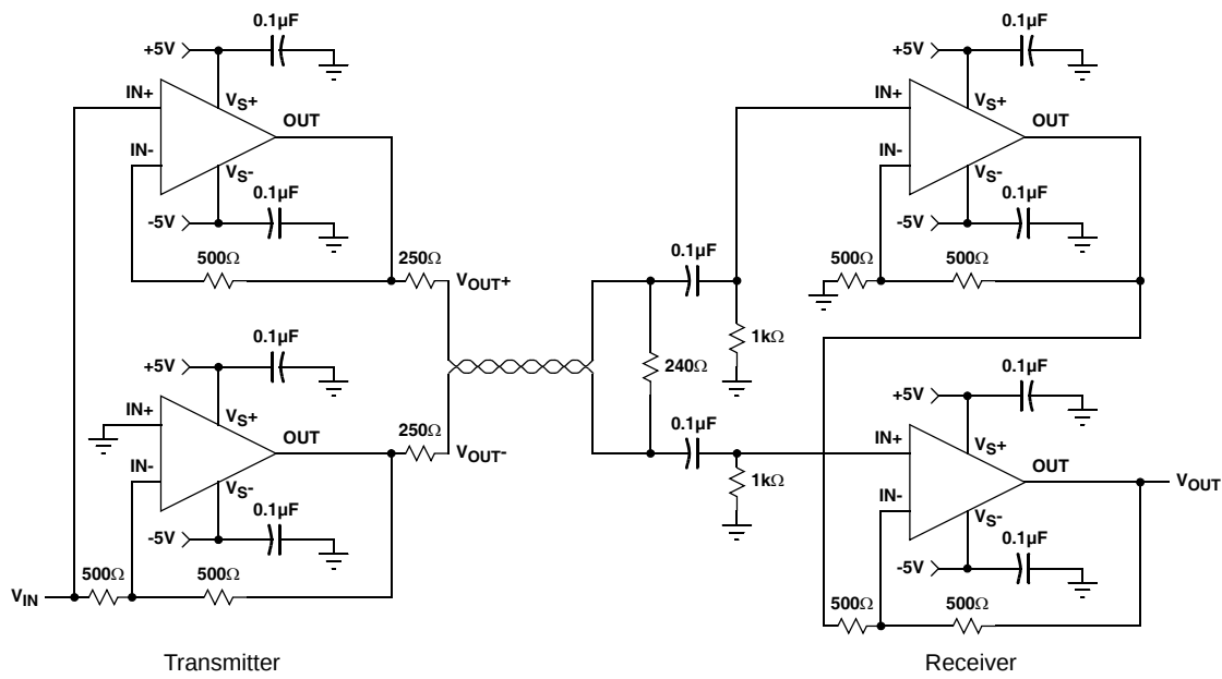
Differential Line Driver/Receiver
