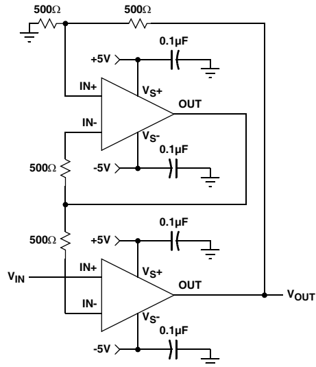
Fast-Settling Precision Amplifier
