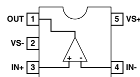
EL5193 (5 LD SOT-23) TOP VIEW
