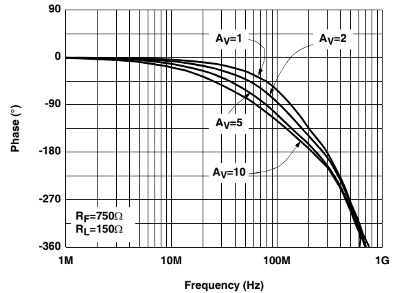
Non-Inverting Frequency Response (Phase) SO8 Package
