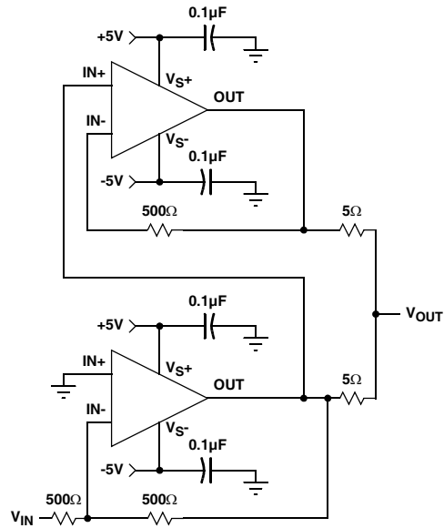
Inverting 200mA Output Current Distribution Amplifier
