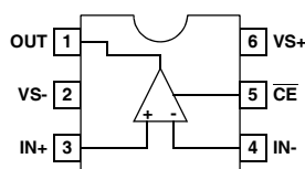
EL5193A (6 LD SOT-23) TOP VIEW
