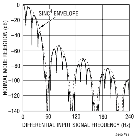
Figure 10. LTC2444/LTC2445/LTC2448/LTC2449 Normal Mode Rejection (Internal Oscillator)
