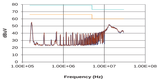
MTC2S2403MC
