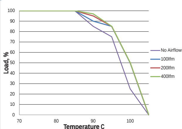
MTC2S2412MC- 24Vin
