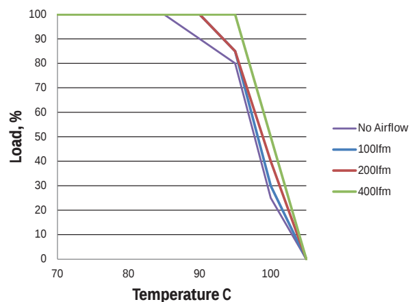
MTC2S1205MC- 9Vin
