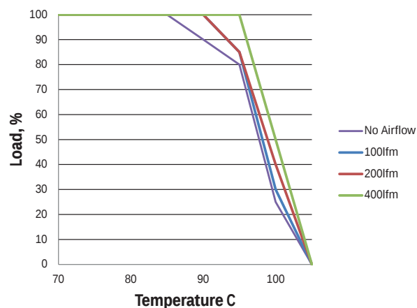
MTC2S1205MC- 12Vin
