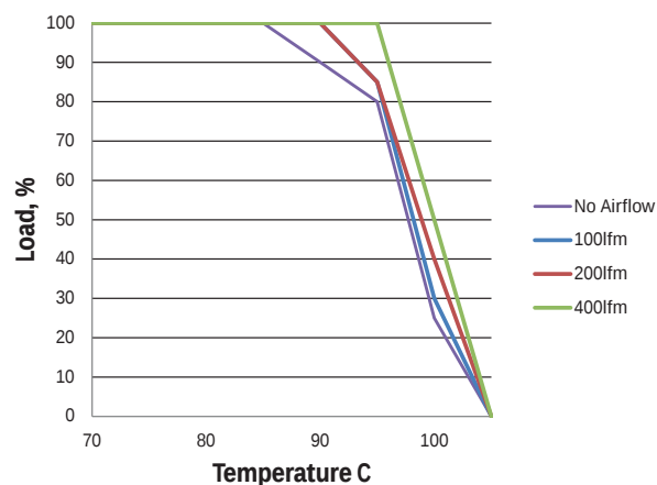
MTC2S1205MC- 18Vin
