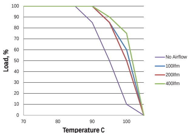
MTC2S1203MC - 12Vin
