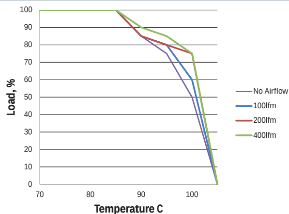
MTC2S2403MC- 24Vin
