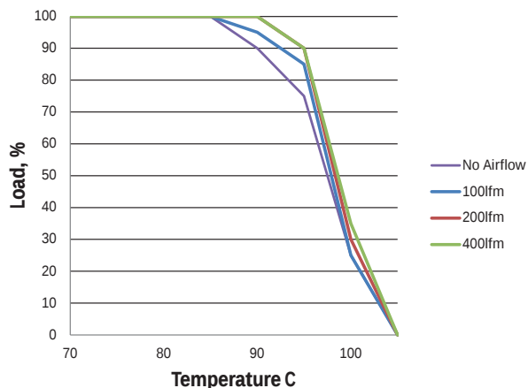
MTC2S2405MC- 24Vin
