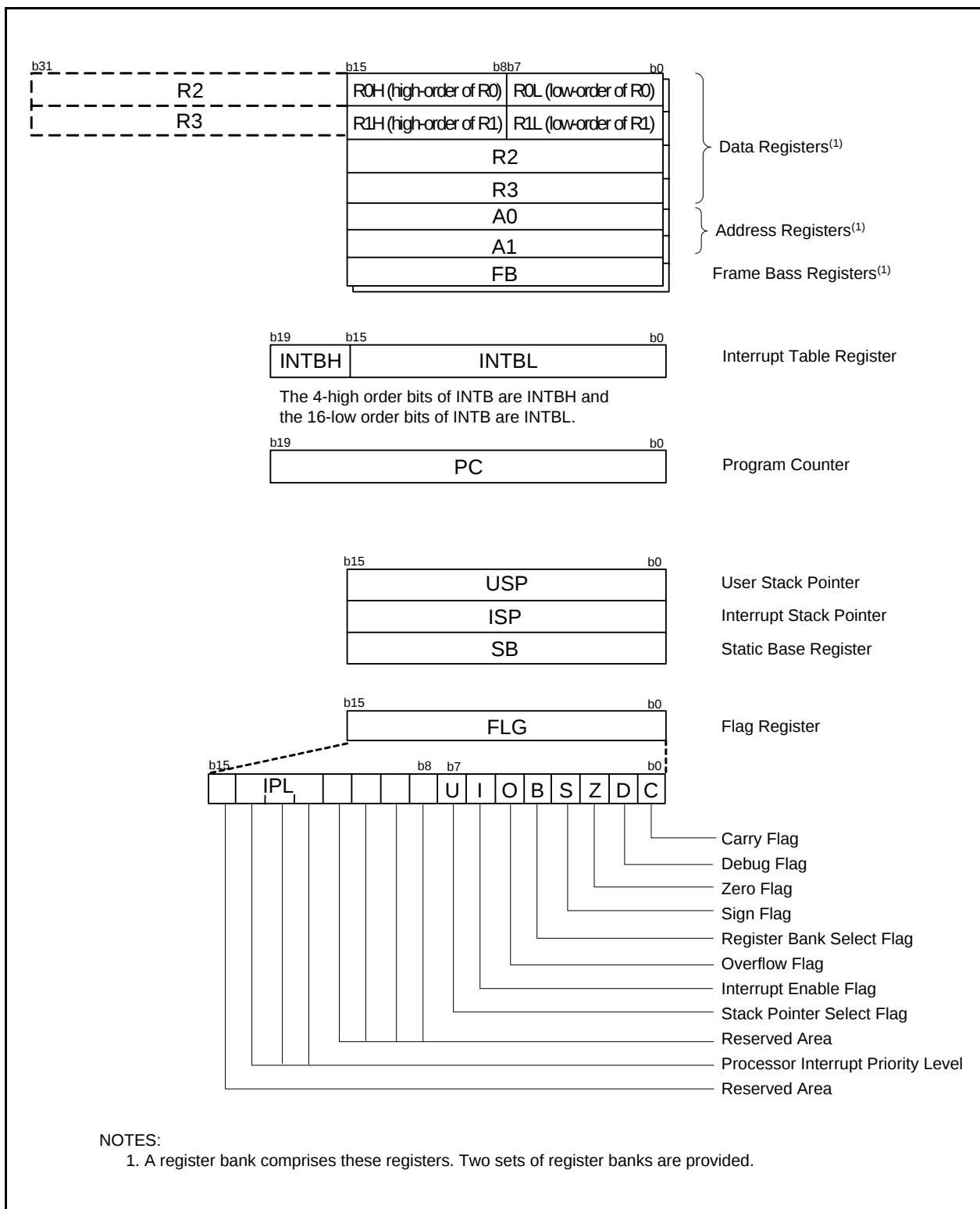
Figure 2.1 CPU Register
