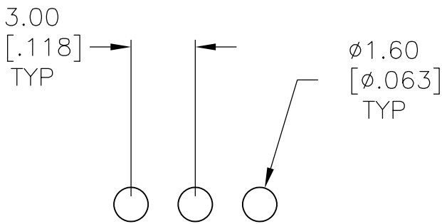
RECOMMENDED HOLE LAYOUT
