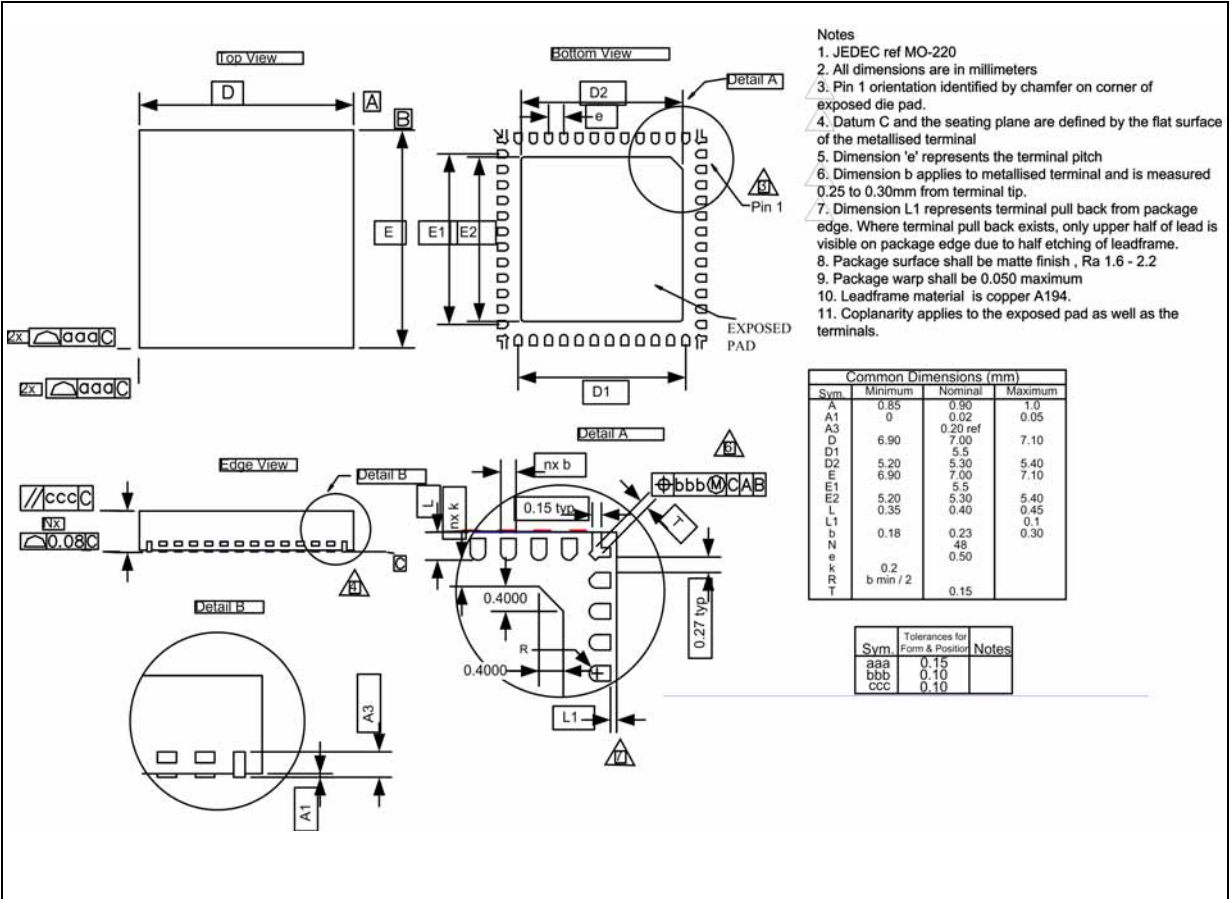
Figure 17. Package drawing
