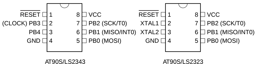
PDIP/SOIC
