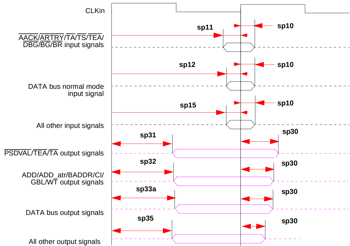
Figure 9. Bus Signals
