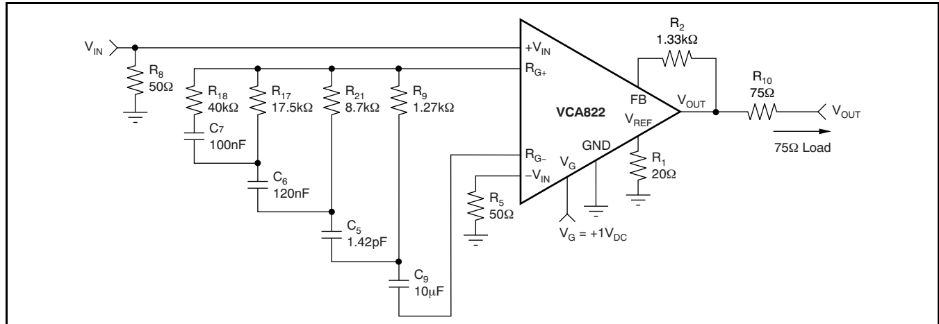
Figure 85. Differential Cable Equalizer
