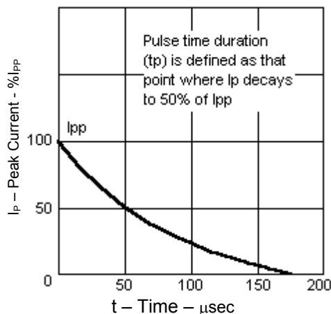
FIGURE 2 Pulse Wave Form (1.2 x 50μs) NOTE: In MIL-STD-1399, Section 300A the source impedance is assumed to be 5ohms at 100 to 200kHz of shipboard electrical power systems.
