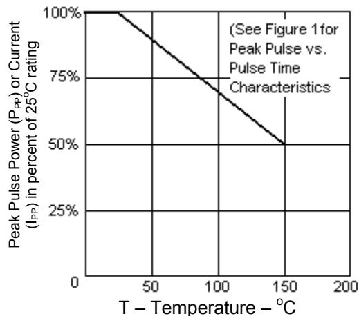
FIGURE 3 Derating Curve NOTE: Maximum operating and storage temperature is 150°C.
