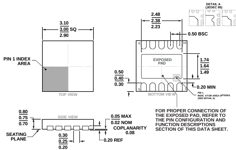
Figure 49. 10-Lead Lead Frame Chip Scale Package [LFCSP] 3 mm × 3 mm Body and 0.75 mm Package Height (CP-10-9) Dimensions shown in millimeters
