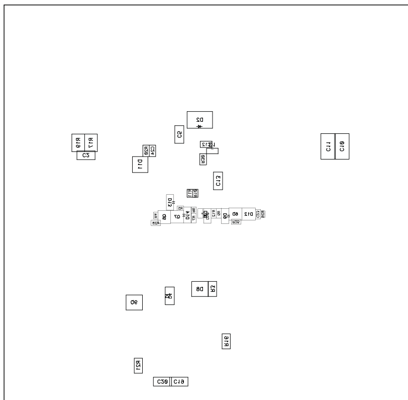
Figure 7. Bottom Assembly
