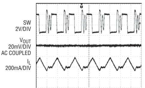
Discontinuous Operation
