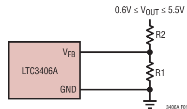
Figure 1. Setting the LTC3406A Output Voltage
