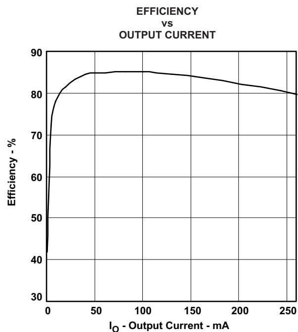
Figure 2. TPS61081 Efficiency With V_{IN} = 3.6 V and VLCF5020T-4R7N1R7-1 Inductor
