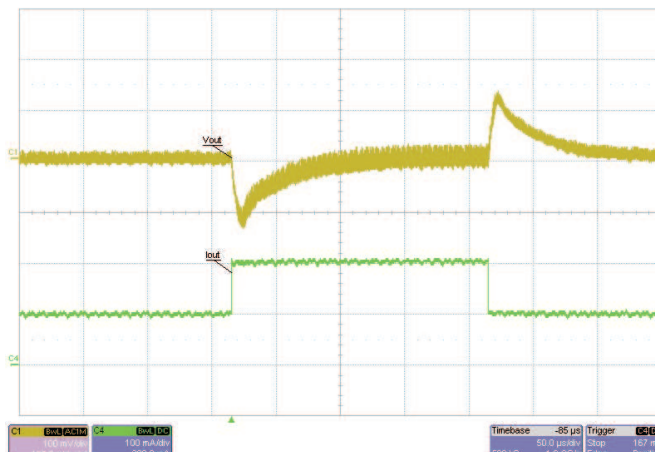
Figure 4. Load Transient Response From 100 mA to 200 mA With C_4 = 10 \mu\text{F} and C_3 = 82 \text{ pF}
