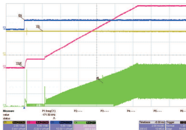
Figure 3. TPS61080 Start-Up With V_{IN} = 3.6 V and I_{OUT} = 50 mA
