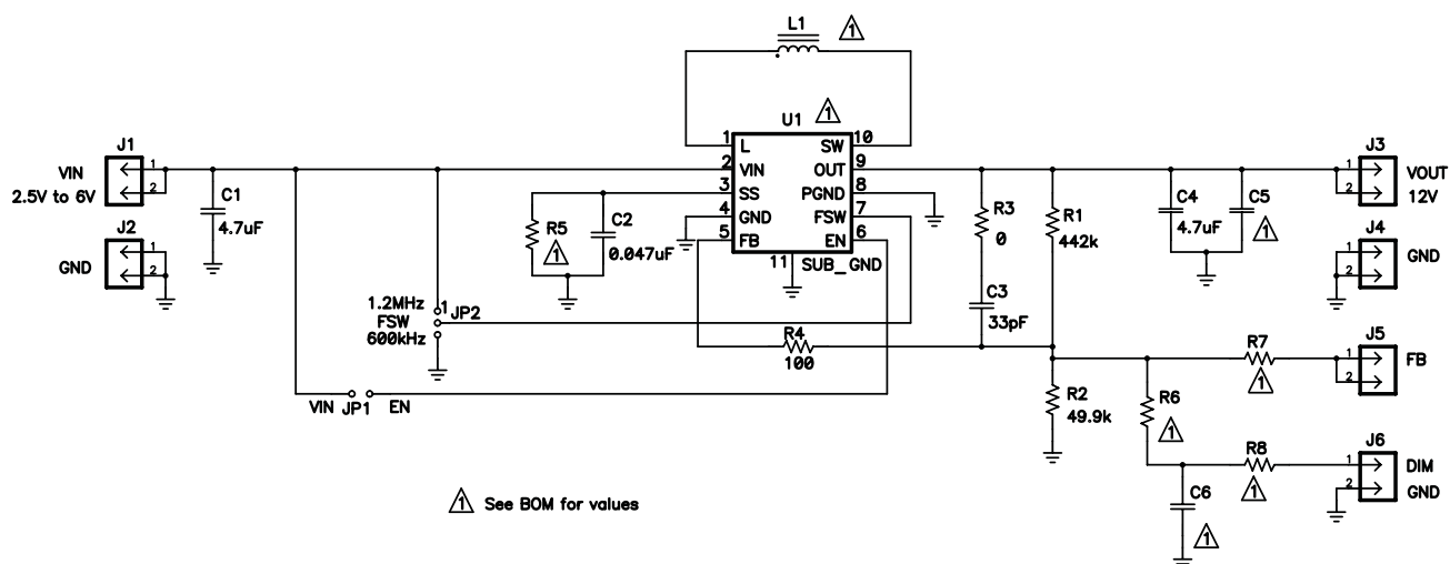
Figure 8. TPS6108xEVM-147 Schematic
