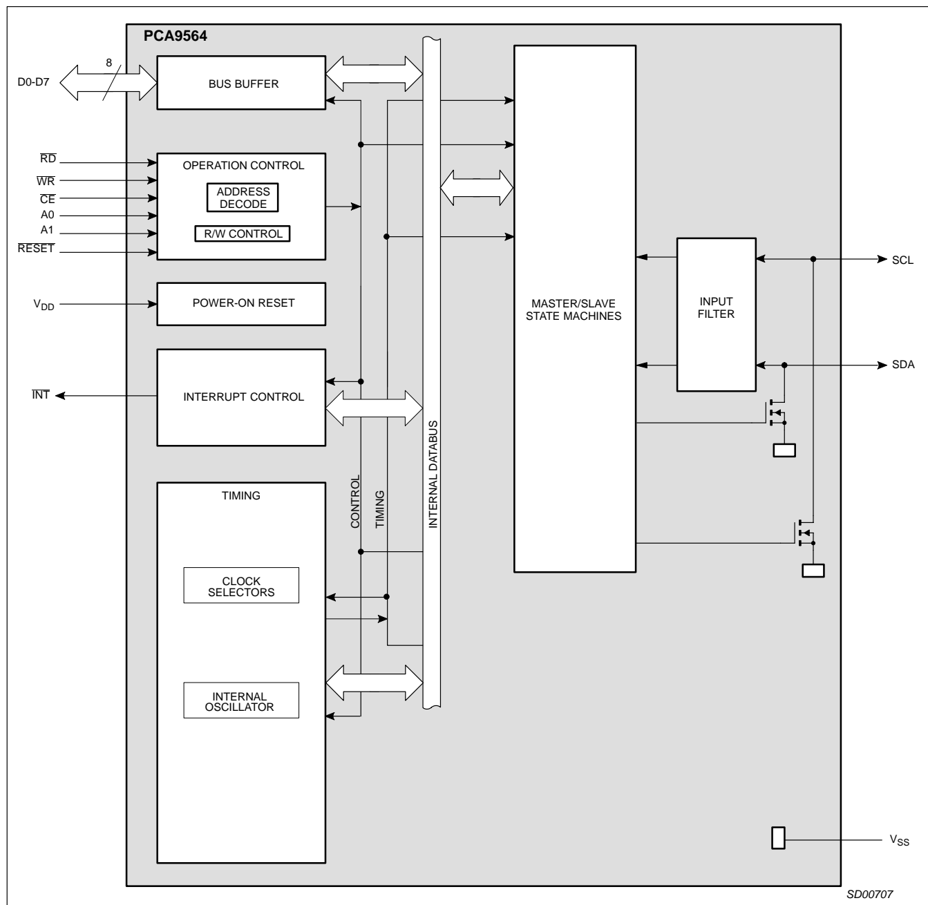
Figure 1. Block diagram
