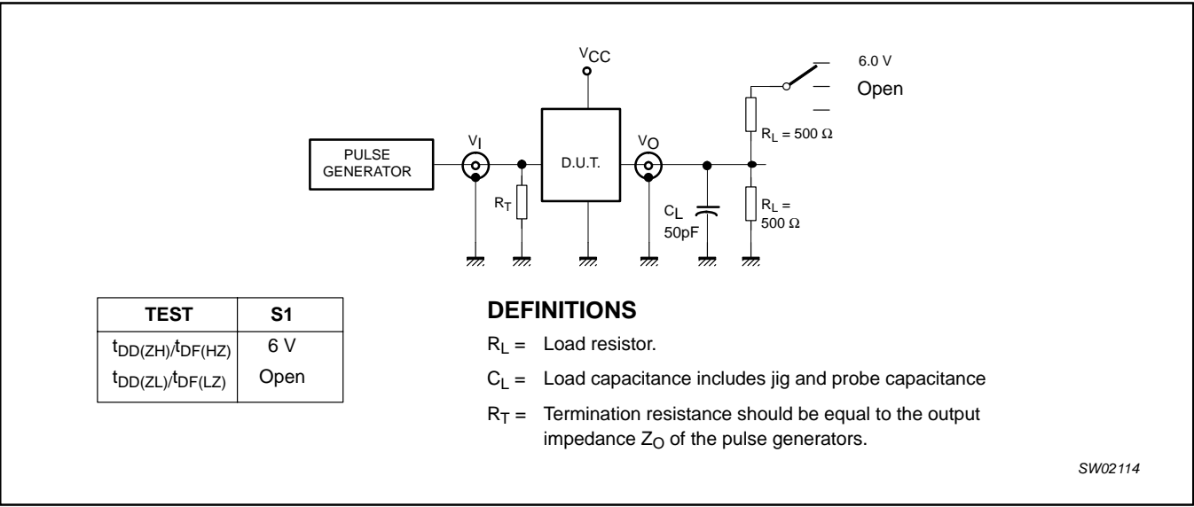
Figure 22. Test circuitry for switching times
