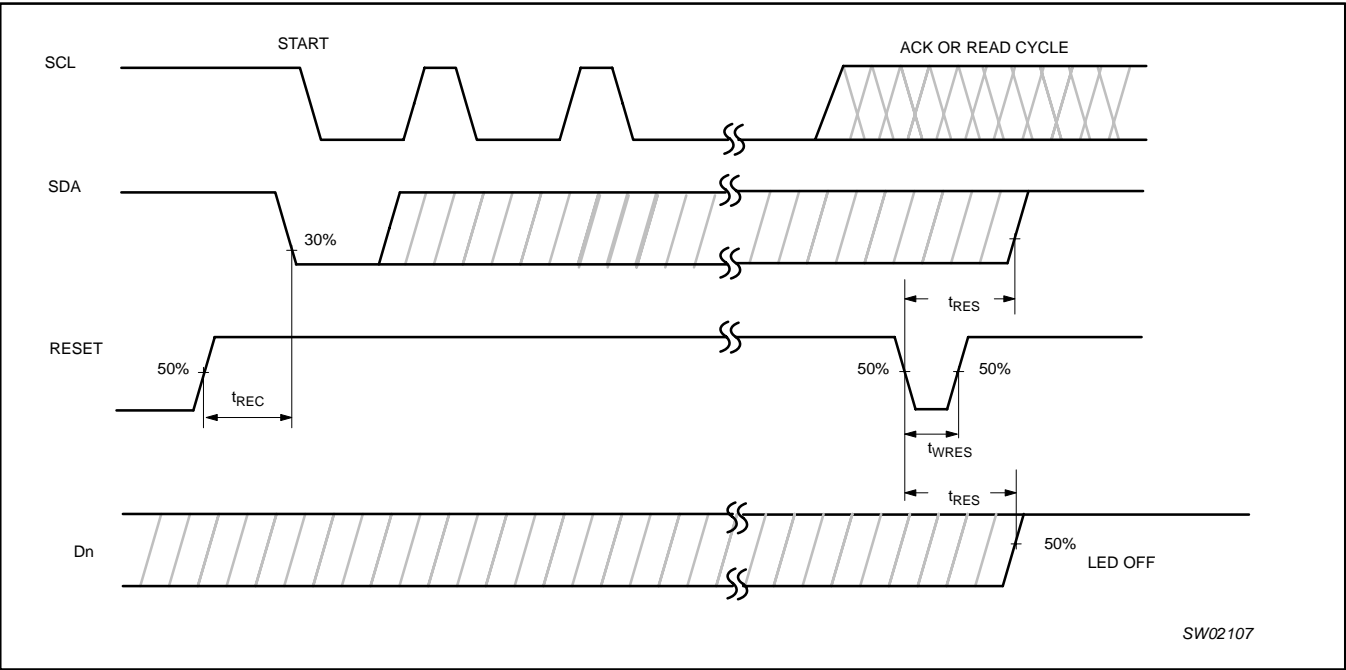
Figure 19. Reset timing
