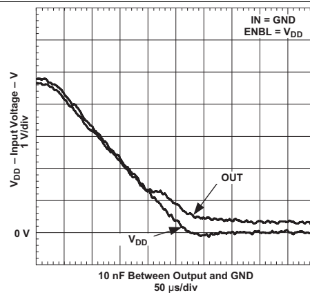
Figure 20. Output Behavior vs V_{DD} (UCC27321-Q1)
