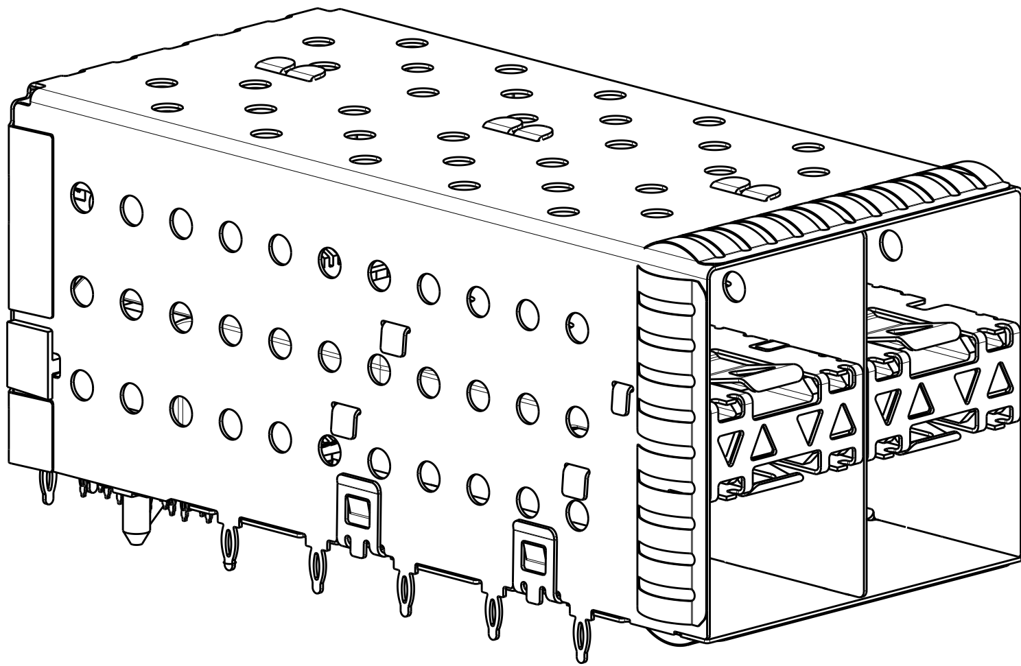
2007637-1, 2007637-5 AND 1-2007637-5 SCALE 3:1
