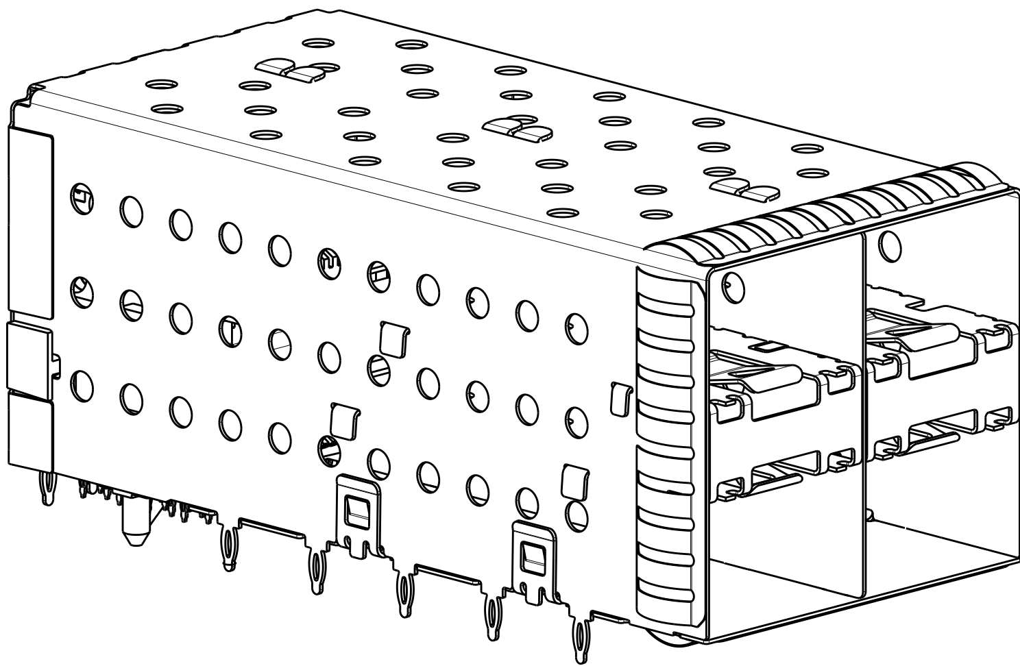
2007637-4, 2007637-8 AND 1-2007637-8 SCALE 3:1
