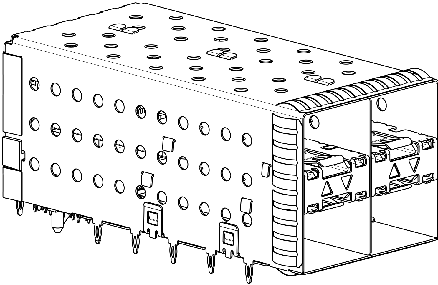
2007637-2, 2007637-6 AND 1-2007637-6 SCALE 3:1
