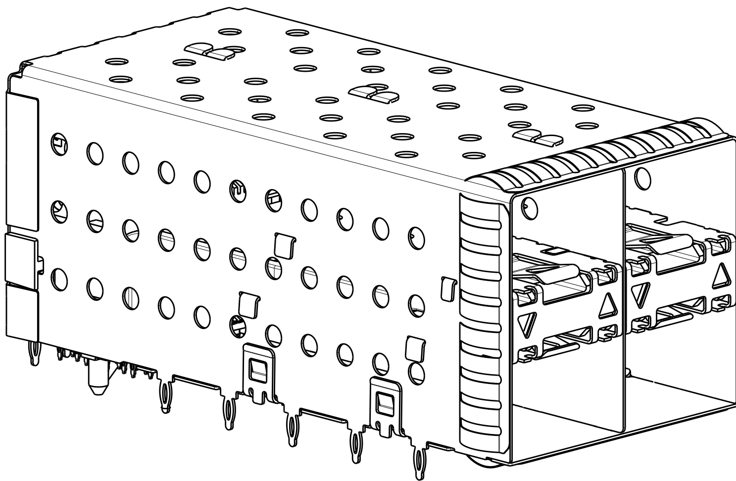
2007637-3, 2007637-7 AND 1-2007637-7 SCALE 3:1
