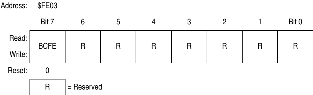
Figure 9-22. SIM Break Flag Control Register (SBFCR)
