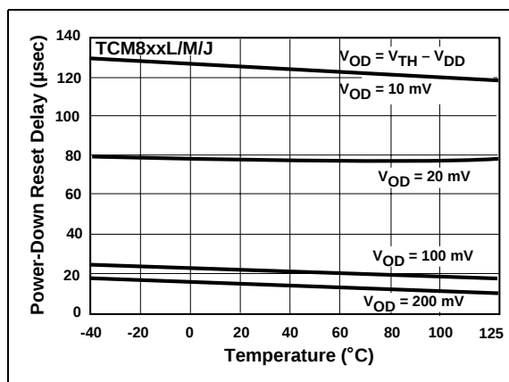
FIGURE 3-6: Power-Down Reset Delay vs. Temperature, SOT-23.
