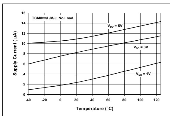
FIGURE 3-5: Supply Current vs. Temperature, SC-70.
