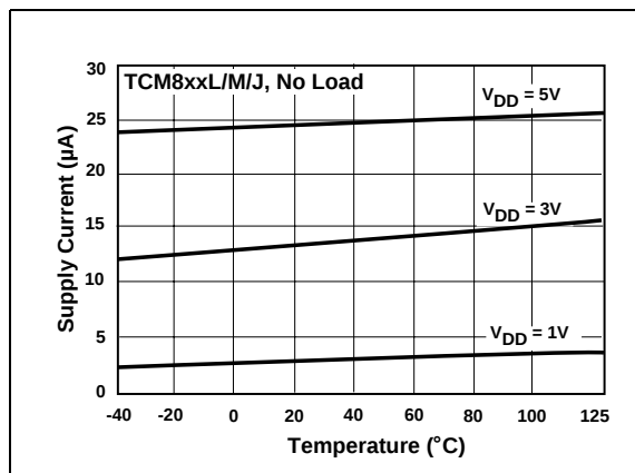
FIGURE 3-4: Supply Current vs. Temperature, SOT-23.
