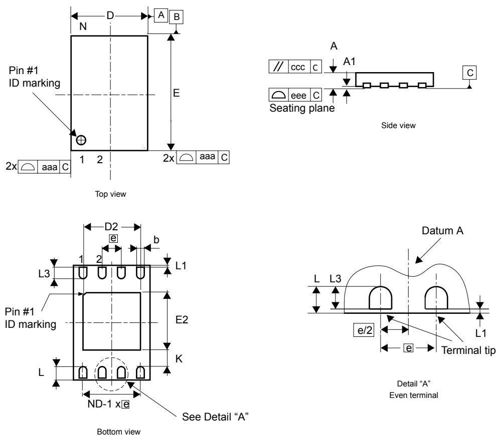
Figure 27. UFDFPN8 - Outline
