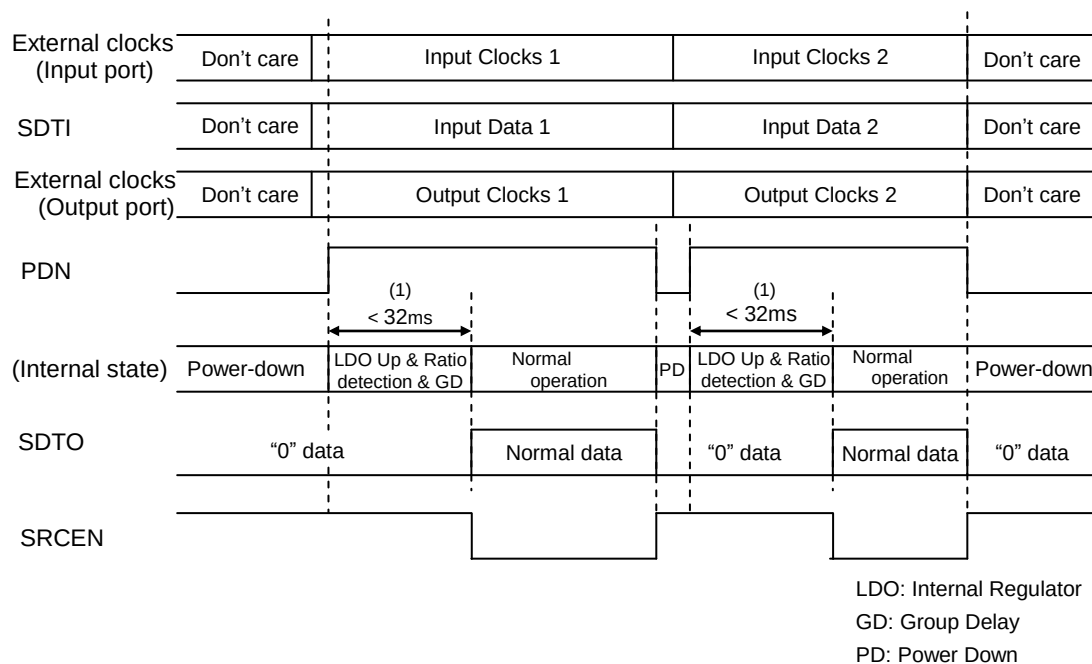
Figure 39. System Reset 1
