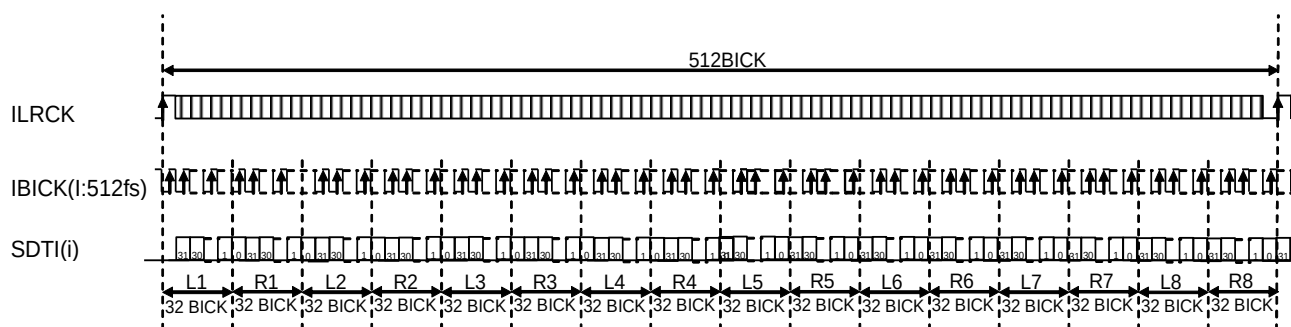
Figure 25. Mode7 Timing (32-bit I²S TDM512fs)
