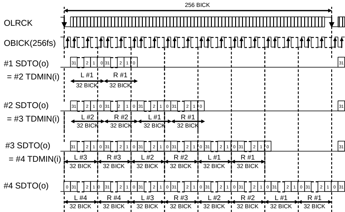
Figure 32. TDM 256 Mode 32bit I 2 S Compatible Timing at Slave Mode
