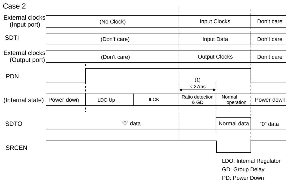
Figure 40. System Reset 2
