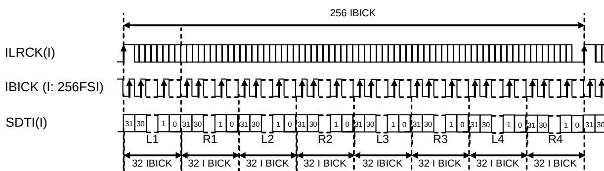
Figure 22. Mode4 Timing (32-bit MSB TDM256fs)
