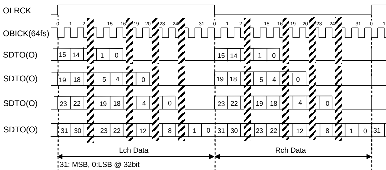
Figure 29. TDM 256 mode 32bit MSB Justified Timing at Slave Mode
