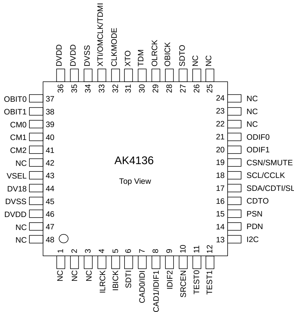
Figure 2. Pin Layout
